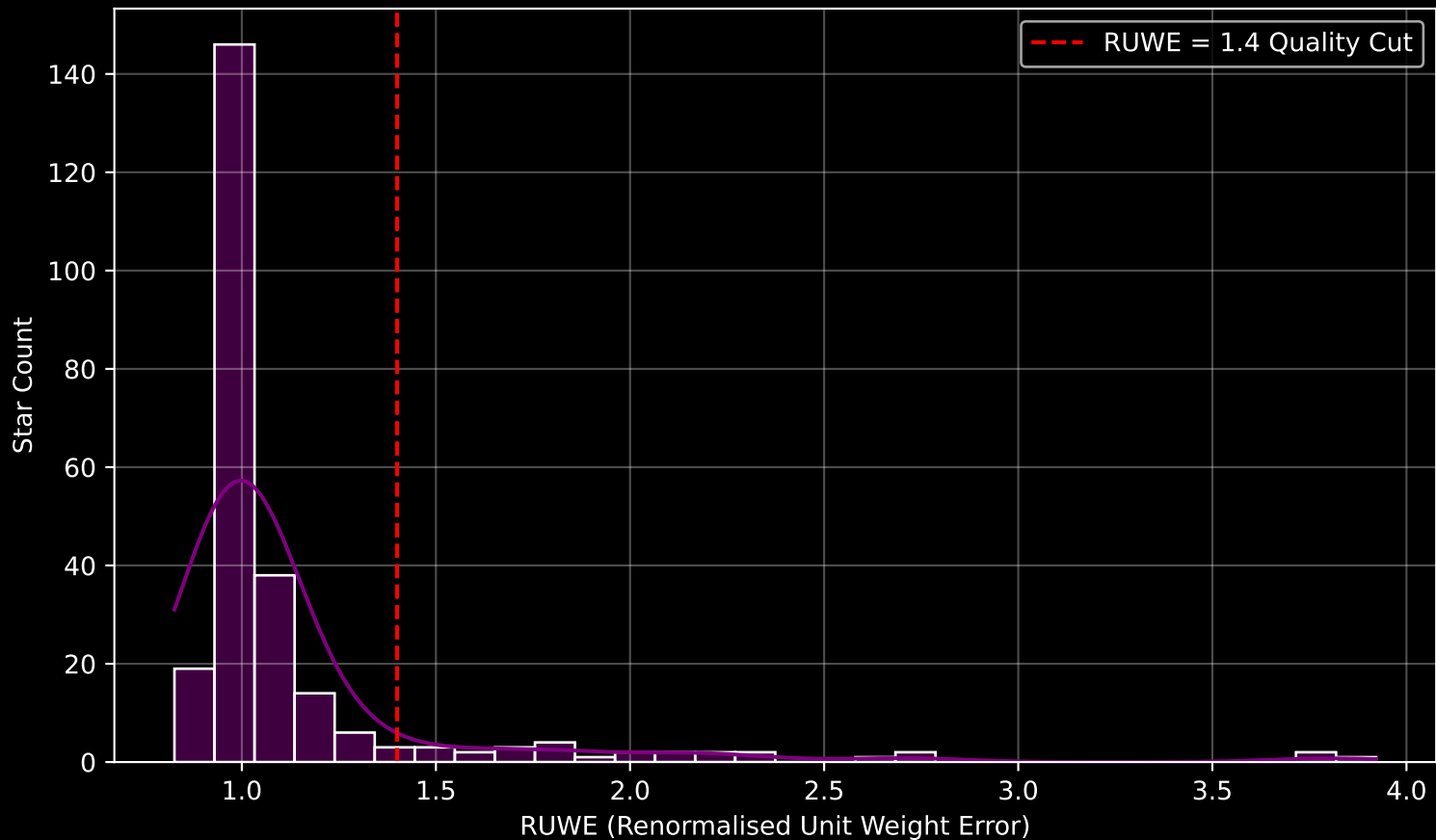
GALAH DR4 Field [1615] RUWE Distribution (n= 253)
