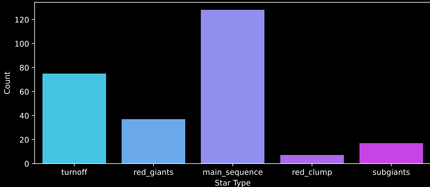
GALAH DR4 Field: [1615] Count plot of Star Type
