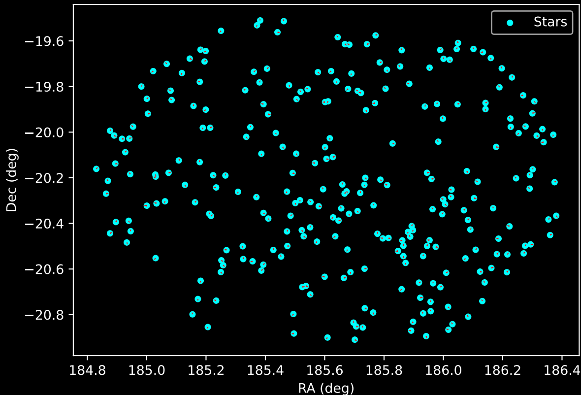
GALAH DR4 Field: [1615] Proper Motion Vectors for Gaia Star Field (n= 264)
